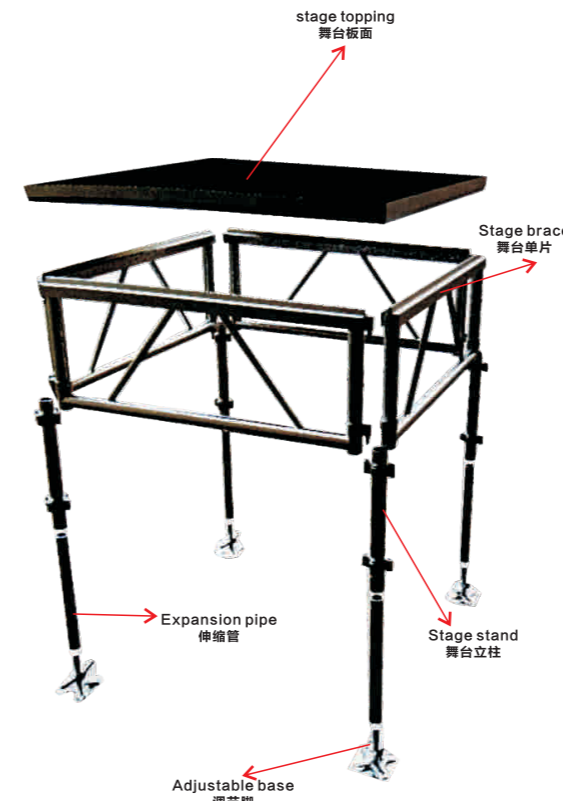
GF-244 1220*2440mm Aluminium assembly stage
