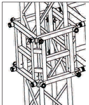
3.方套/Sleeve Block
