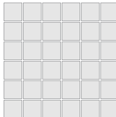
单粒 Chipsize: 45X45mm 联长 Sheetsize: 291X291mm 灰缝 Joint Width: 3.5mm
