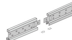
铝大方槽龙骨接驳示意图 Drawing of Connection of Aluminum Square-groove Carrier
