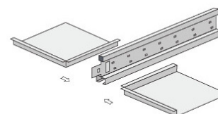
明架方板安装示意图 Installation Illustration of Lay-in Ceiling
