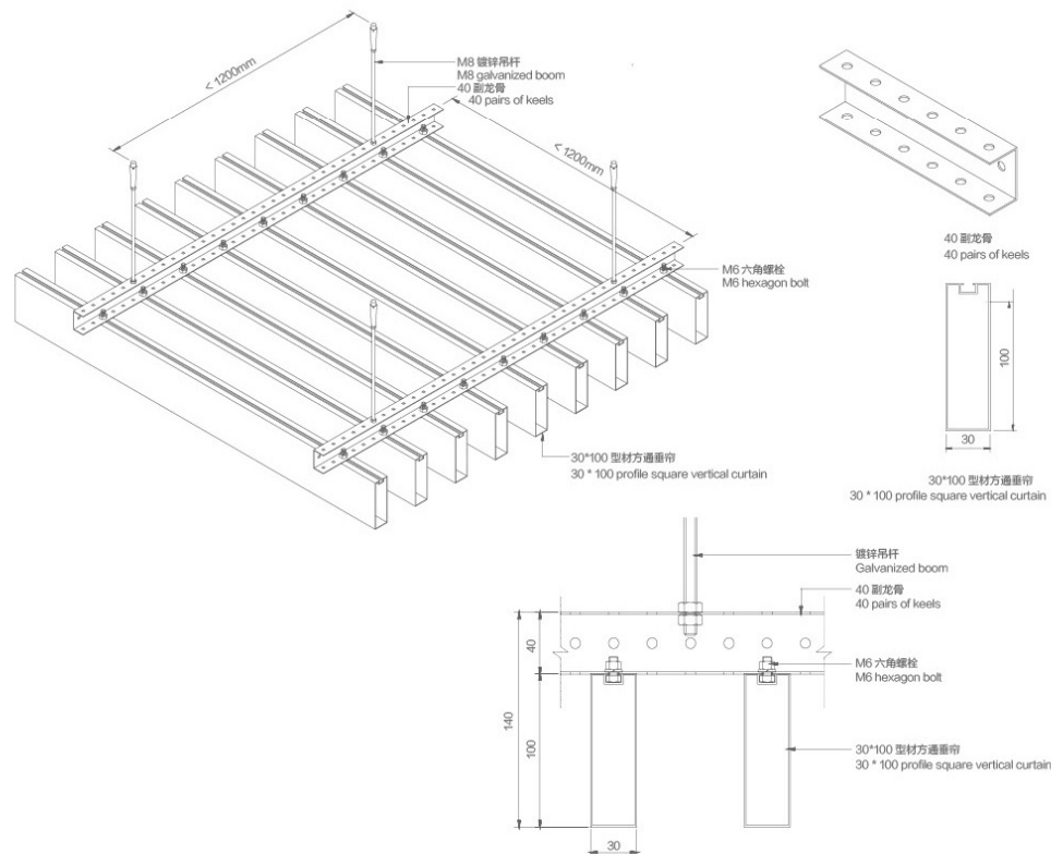
INSTALLATION STRUCTURE DIAGRAM OF ALUMINUM PROFILE CURTAIN WALL 型材方通安装结构图
