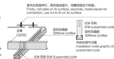
GRAPHIC ILLUSTRATION CONNECTION POINT OF PLATE TO PLATE 板与板连接节点图
