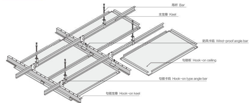
MOUNTING STRUCTURE OF HOOK BOARD SUSPENDED CEILING 勾搭板吊顶安装结构图
