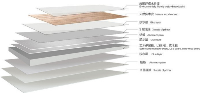
STRUCTURE OF COMPOSITE BOARD 复合板结构图
