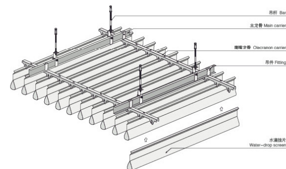
INSTALLATION STRUCTURE DIAGRAM OF WATER DROP HANGING PIECE 水滴挂片安装结构图
