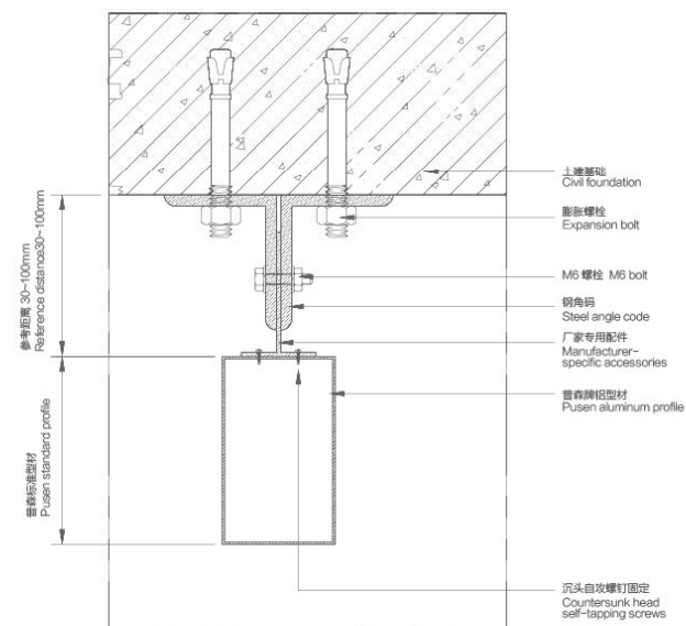
INSTALLATION STRUCTURE DIAGRAM OF ALUMINUM PROFILE CURTAIN WALL 铝型材幕墙安装结构图
