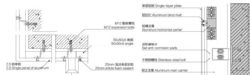
INTERNAL CORNER INSTALLATION ILLUSTRATION TO ALUMINUM SINGLE PLATE 铝单板内部转角安装实例
