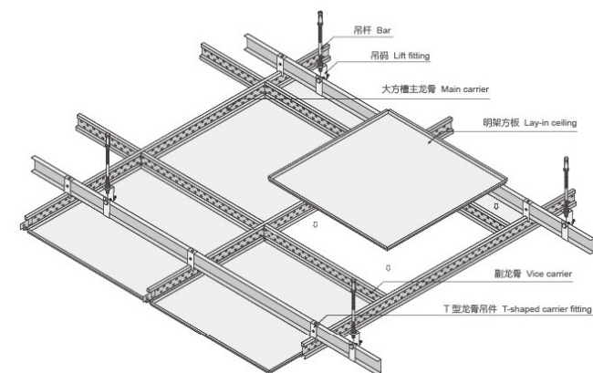
STRUCTURE DIAGRAM OF LAY-IN CEILING 明架方板安装结构图
