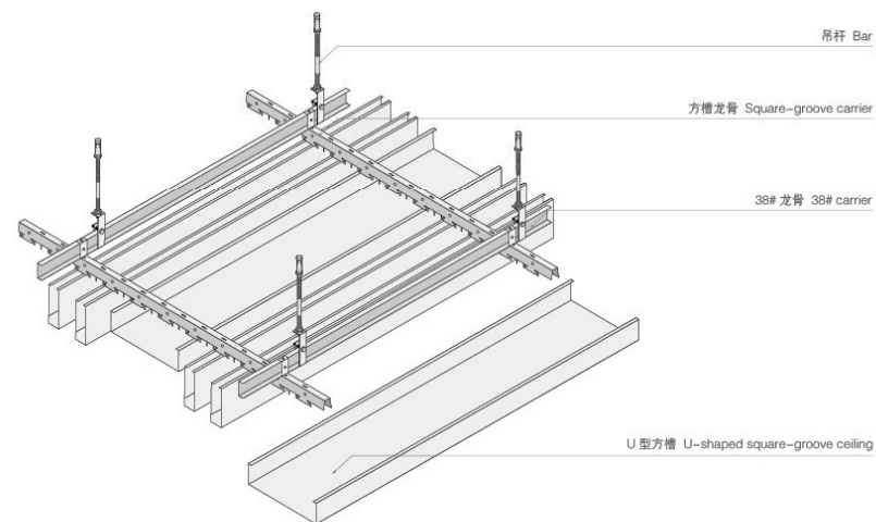
STRUCTURE DIAGRAM OF U-SHAPED SQUARE-GROOVE CEILING U 型方槽安装结构图
